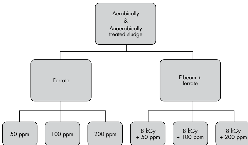
Figure 1. Schematic Representation of the Experimental Design Involving Ferrate and Ferrate Combined with E-beam.
